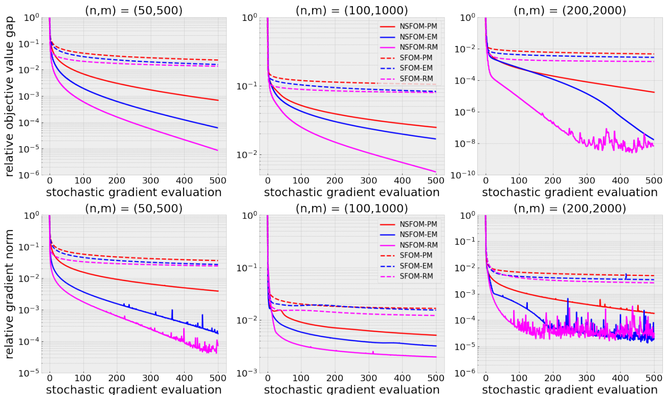
Figure 1: Convergence behavior of the relative objective value gap (first row) and relative gradient norm (second row) for all methods in solving problem (31).
